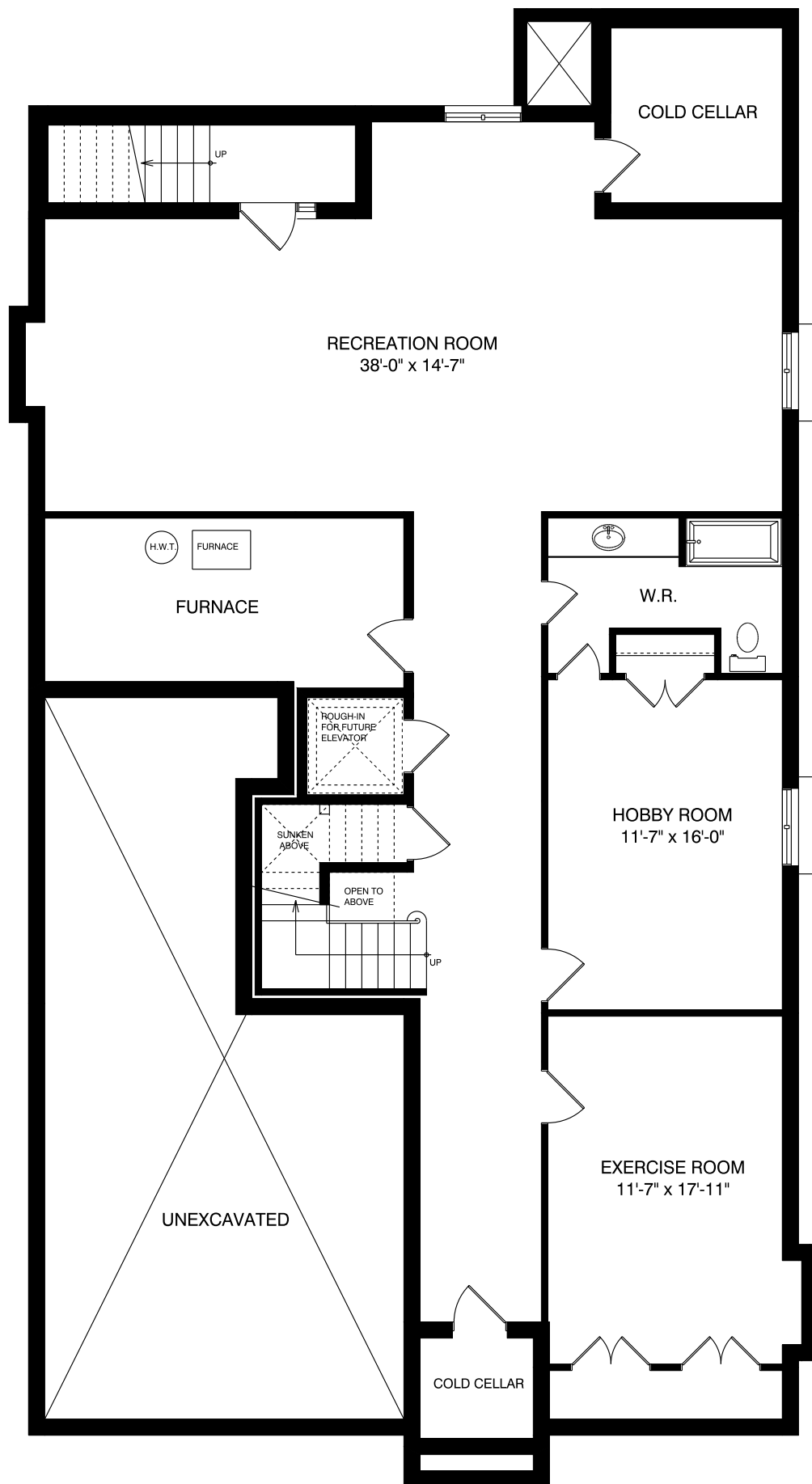
BASEMENT PLAN
